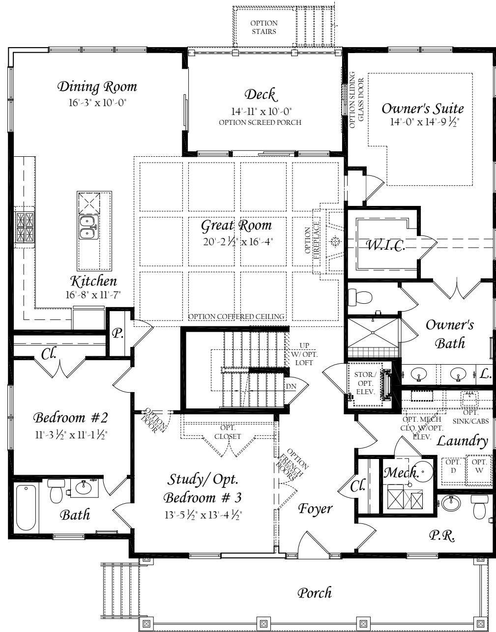
MAIN LEVEL
